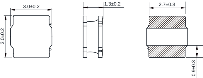
Dimensions: [mm]
