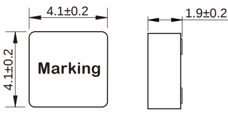
Dimensions: [mm]
